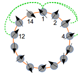
FIG. 1. Practical construction of a Lace network for N = 14 , k = 2 , and r = [\sqrt{N}] = 3 . The starting configuration is in orange and the dotted green links are the possible rewirings allowed within the range r .
