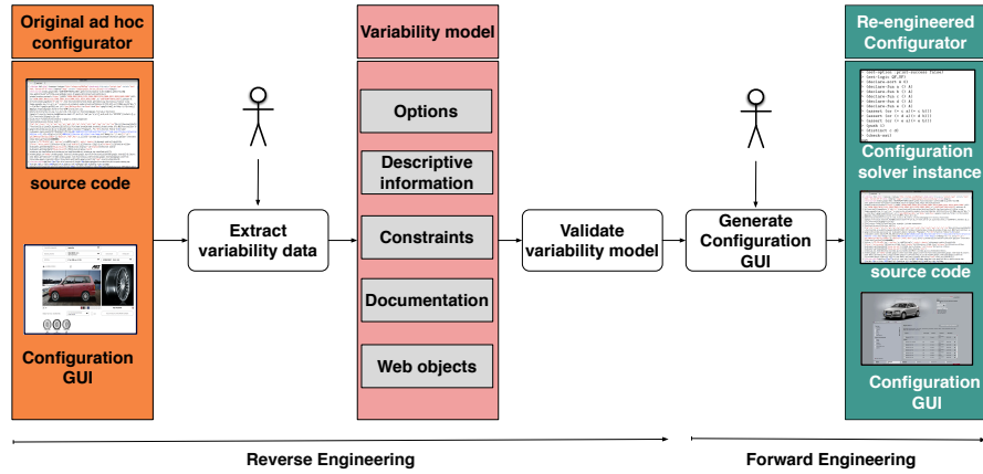
Fig. 10: Re-engineering process for configurators
