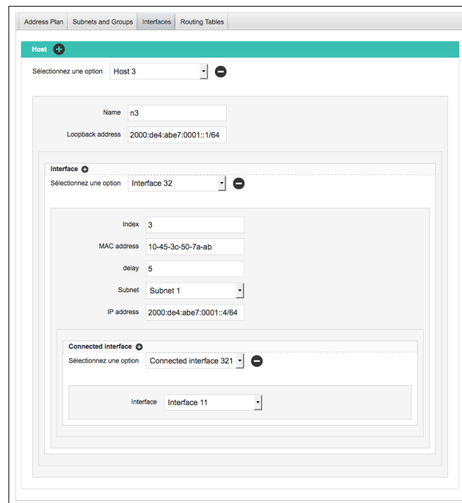
Fig. 8: Interfaces tab of the HTML configurator for IPv6 addressing plans
