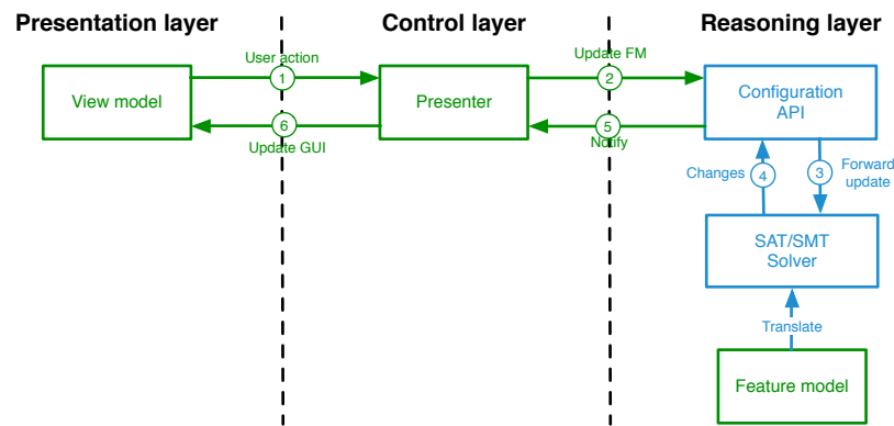
Fig. 3: An MVP architecture for configurators
