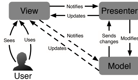
Fig. 2: Model-view-presenter architecture
