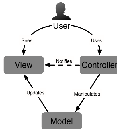
Fig. 1: Model-view-controller architecture
