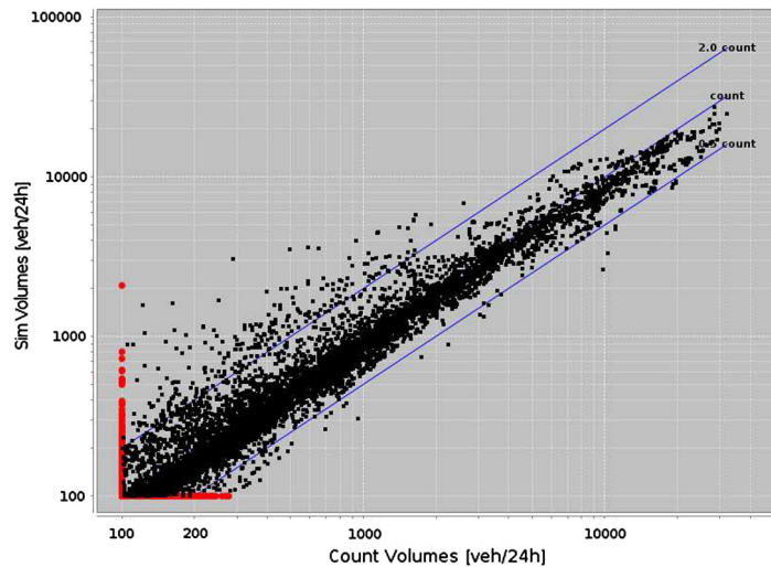
Fig. 16. Strategic agents traffic counts ( x axis) against MATSim traffic counts ( y axis). Each dot represents a link and the daily traffic volume predicted by the proposed model and MATSim. Pearson correlation coefficient \rho = 0.951 , adjusted R^2 = 0.905 .
