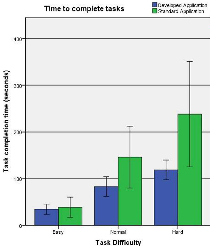
FIGURE 4 | Time to complete tasks by difficulty level and application.
