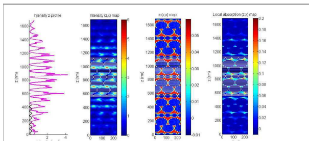
Fig. 6 (From left to right) Intensity z -profile at the center of unit cell (magenta curve) and cross section ( x,z ) maps of field intensity, imaginary part of dielectric constant and local absorption in a close-packed IO slab with D=115 nm (red-edge-tuned). Profiles and maps were calculated at \lambda=361 nm for non-polarized light impinging perpendicularly to the slab. Sphere cross sections are shown in the central part of the IO slab as guide for the eyes. Intensity z -profile in the reference slab is also shown (black curve).
