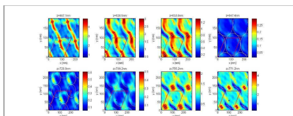
Fig. 7 Cross section ( x,y ) maps of field intensity at various depths in red-edge-tuned (top row) and blue-edge-tuned (bottom row,) close-packed IO slabs with, respectively, D=115 nm and D=137 nm. Maps were calculated at \lambda=361 nm (top row) and \lambda=359 nm (bottom row) for non-polarized light impinging perpendicularly to the slab. Cross section (centre) of the unit cell is indicated by red parallelogram (black cross). White circles are sphere cross sections.
