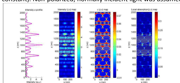
Fig. 8 (From left to right) Intensity z -profile at the center of unit cell (magenta curve) and cross section ( x,z ) maps of field intensity, imaginary part of dielectric constant and local absorption in a close-packed IO slab with D=137 nm (blue-edge-tuned). Profiles and maps were calculated at \lambda=359 nm for non-polarized light impinging perpendicularly to the slab. Sphere cross sections are shown in the central part of the IO slab as guide for the eyes. Intensity z -profile in the reference slab is also shown (black curve).
