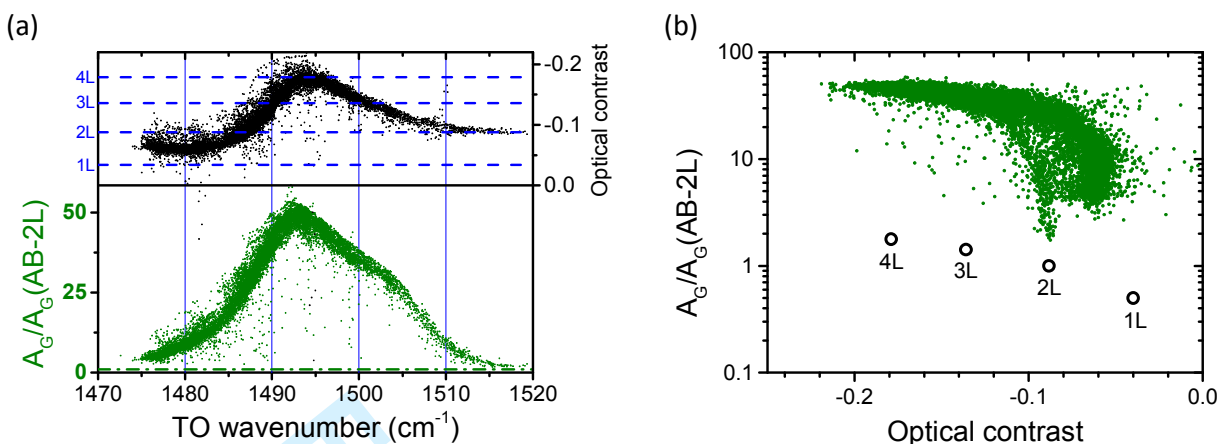
Figure 4: Illustration of the impact of an optical resonance for bilayer graphene (2L) deposited on 300 nm SiO 2 /Si substrate. (a) top panel (black points) optical contrast and bottom panel (green points) A_G relative to the A_G of AB-2L as a function of the TO wavenumber (related to the twist angle between the two layers [47]) measured with a 532 nm laser. The horizontal blue dashed lines in the top panel represents optical contrast of mechanically exfoliated samples 1L to 4L as labelled on the figure. The horizontal green dashed line in the bottom panel highlights the value 1. (b) A_G relative to the A_G of AB-2L as a function of the optical contrast. The green filled dots correspond to data presented in (a) and the black open circles correspond to data obtained on mechanically exfoliated samples (1L to 4L as labelled on the plot) deposited on an equivalent substrate.
