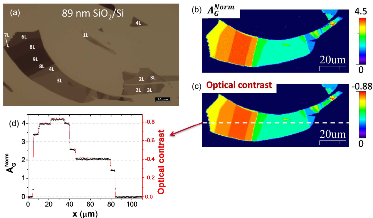
Figure 2: (a) Optical microscopy image of a FLG sample deposited by micromechanical exfoliation on 89 nm \text{SiO}_2/\text{Si} . The number of layers N is labelled as N\text{L} on the corresponding regions of the image and has been determined by spectral microreflection, Raman and laser optical contrast. (b) G band integrated intensity normalized versus the one of HOPG map and (c) Optical contrast map extracted from a Raman/reflection mapping of the sample with a 532 nm laser and a 100x objective. (d) Profile along the white dotted line on (c) of the A_G^{\text{Norm}} (left Y axis) and optical contrast (right Y axis).
