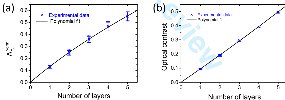
Figure 6: (a) A_G^{Norm} and (b) optical contrast as a function of the number of layers ( N ) measured on mechanically exfoliated samples on soda lime glass (blue dots). The solid black lines are the polynomial fits corresponding to eq. (1) and (2) in the text (coefficients of determination: R^2=0.9998 and R^2=0.9999 for A_G^{Norm} and optical contrast, respectively).
