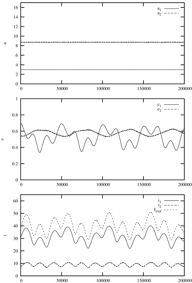
Figure 4. Evolution of the system shown in Fig. 2, after suddenly switching off the migration force (at t = 1 \times 10^6 yr).
