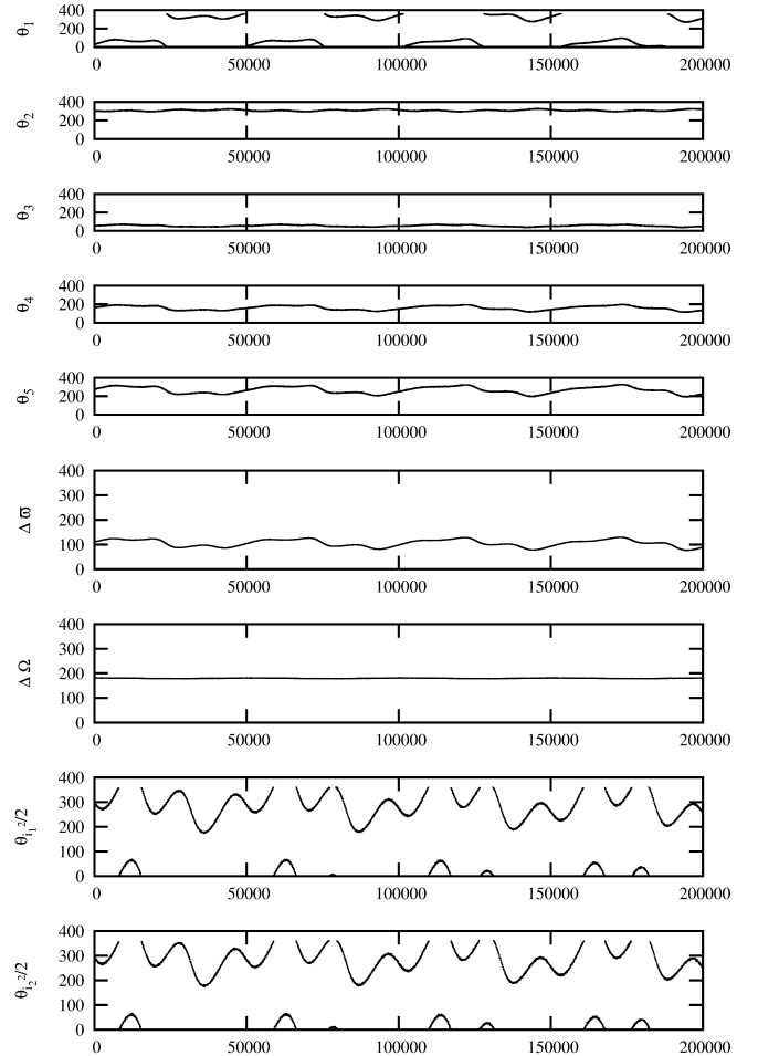
Figure 4. Evolution of the system shown in Fig. 2, after suddenly switching off the migration force (at t = 1 \times 10^6 yr).
