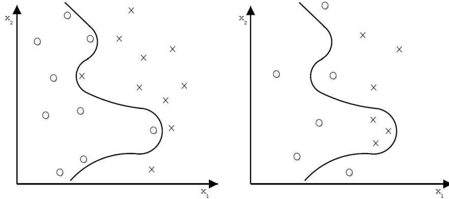
Figure 3.2: Overfitting Illustration
