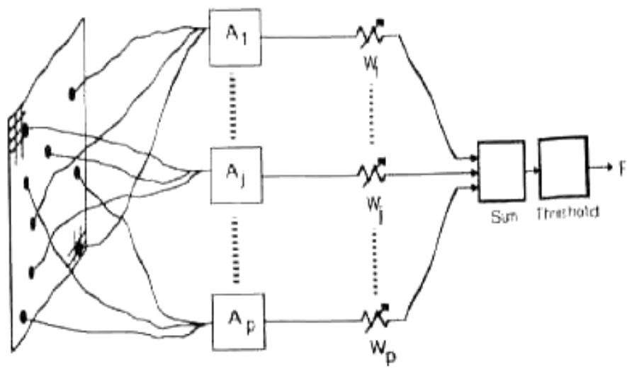
Figure 2.9: Perceptron
