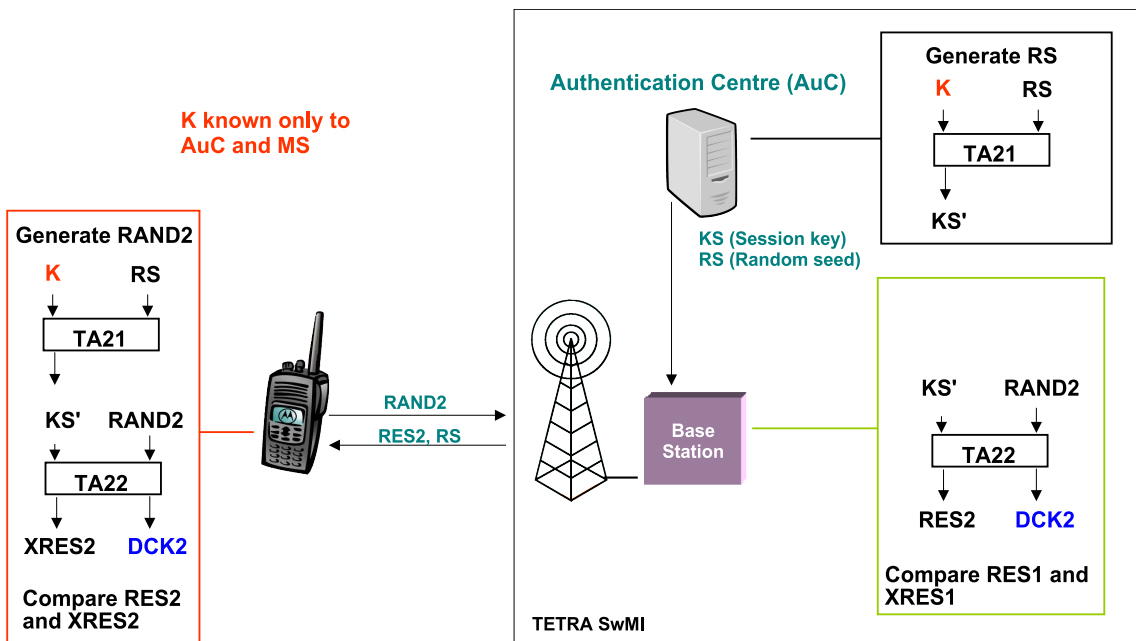
FIG. 8.2 – Authentication infrastructure
