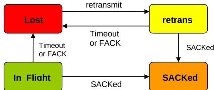
Figure 16: state machine of each packet [11]
