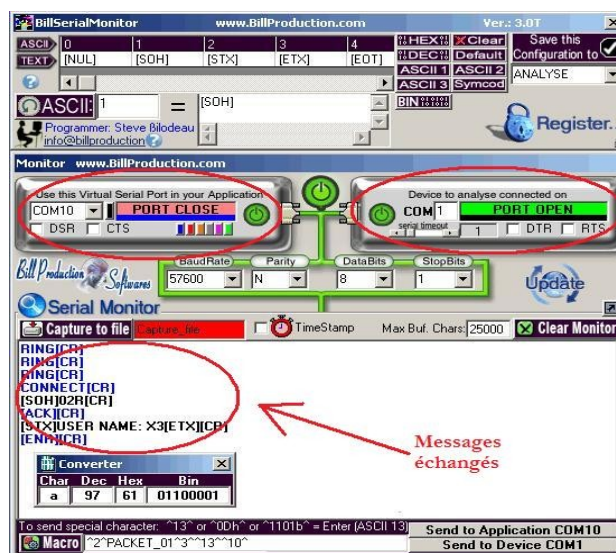
Illustration 15: L'interface de BillSerialMonitor, un programme de monitoring RS-232
