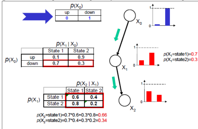
Figure 3.1: Example of a simple Bayesian Network that operates.
