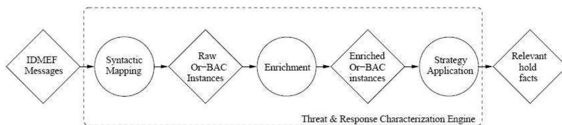
Figure 15: Threat Characterization Engine [7]
