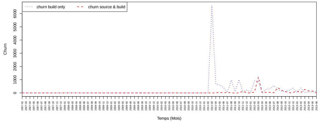
FIGURE 5.7 – Co-churn de Maven de LinuxTools
