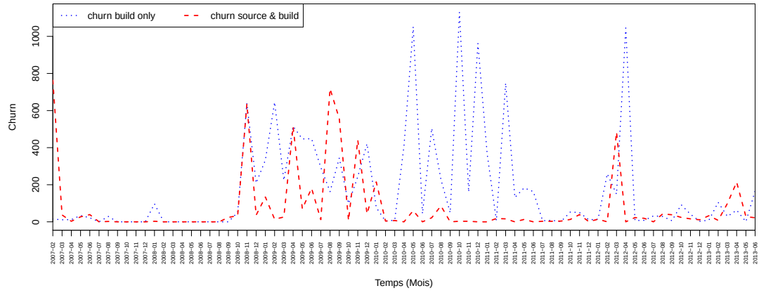
FIGURE 5.6 – Co-churn de Ant de LinuxTools
