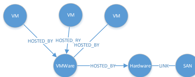
FIGURE 7.4 – Template - Virtualisation
