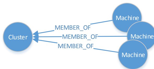
FIGURE 7.5 – Template - Cluster
