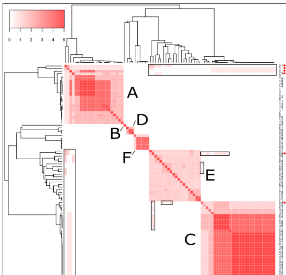
Figure 2 : Conspecificity matrix highlighting the congruence between the five markers, resulting in the delineation of six species (A-F) among the 82 A. vaga individuals sequenced. This matrix was obtained computing, for each pair of individuals, a conspecificity score equal to the number of independent markers supporting the hypothesis of their conspecificity, , then reordering the rows and columns to maximize the scores along the diagonal. The highest scores (5 out of 5) are shown in red, whereas the lowest scores are shown in white (and the intermediate scores in various shades of pink). The black frames indicate incongruent species assignment for six individuals (red arrows). The twelve individuals (Ind38-47, 54 and 55) isolated from the same patch and harbouring the same COI haplotype 12 form one dense red block on the bottom right corner of the matrix.
