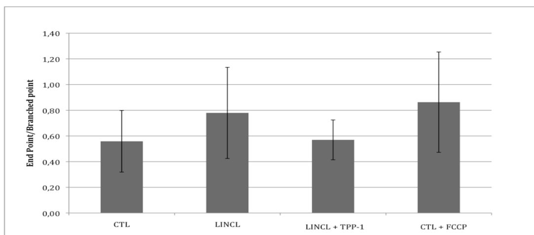
Figure 3.5 : Quantification de la fragmentation du r  seau mitochondrial (Ending Point/Branching Point)
