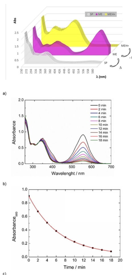
Figure 4. UV/Vis absorption spectroscopy data of MEH + _NO 2 . a) A fresh solution of the protonated merocyanine (10 −4 M in CH 3 CN) is yellow (MEH + ) and is stable if kept in the dark. It turns violet (ME) if passed through a plug of solid sodium carbonate (−H + ). b) The resulting ME form (violet solution, \lambda_{\text{max}} = 558\text{ nm} ) returns to the stable colorless closed SP isomer within 20 min at room temperature. c) Exponential decay of SP_NO 2 ( t_{1/2} = 4.68 \pm 4\text{ min} ).
