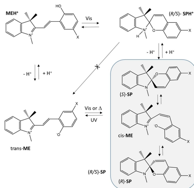
Figure 1. Four-state molecular system involving spiropyrans. (R/S)-SP (SP from here on): spiropyran; MEH + : protonated merocyanine; (R/S)-SPH + (SPH + ): protonated spiropyran; ME: merocyanine. Nitro-substituted compound (X = NO 2 ) has been extensively studied. [2] Compounds included in this study correspond to X = NO 2 and Br.
