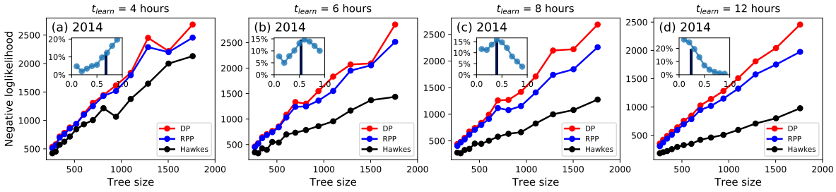
Figure 8: Negative likelihoods for the predicted activity of large trees in 2014. The learning time t_{learn} for parameters evaluation is (a) 4, (b) 6, (c) 8 and (d) 12 hours. The insets show the distribution of the fraction of activity that remains to predict after the learning phase.
