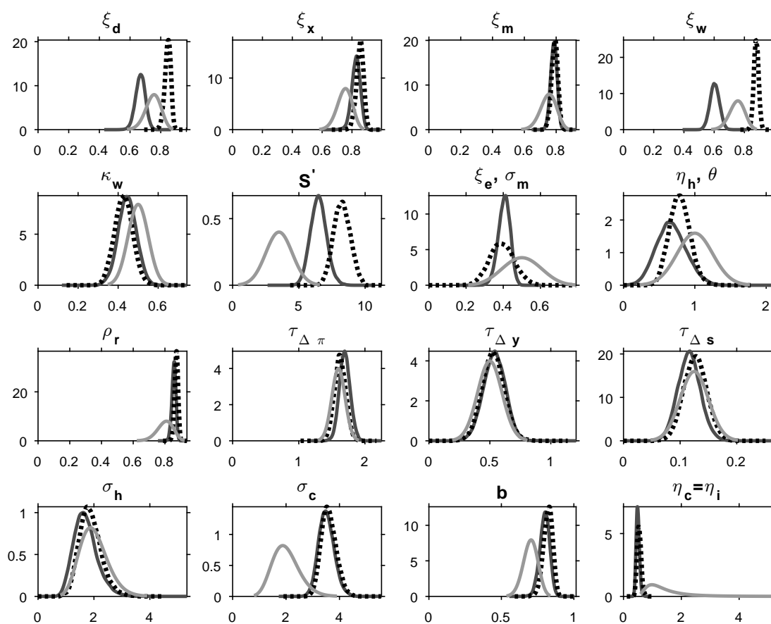
Figure 3.4: Prior and posterior densities - domestic parameters
