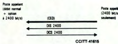
FIGURE V-10/T.30
