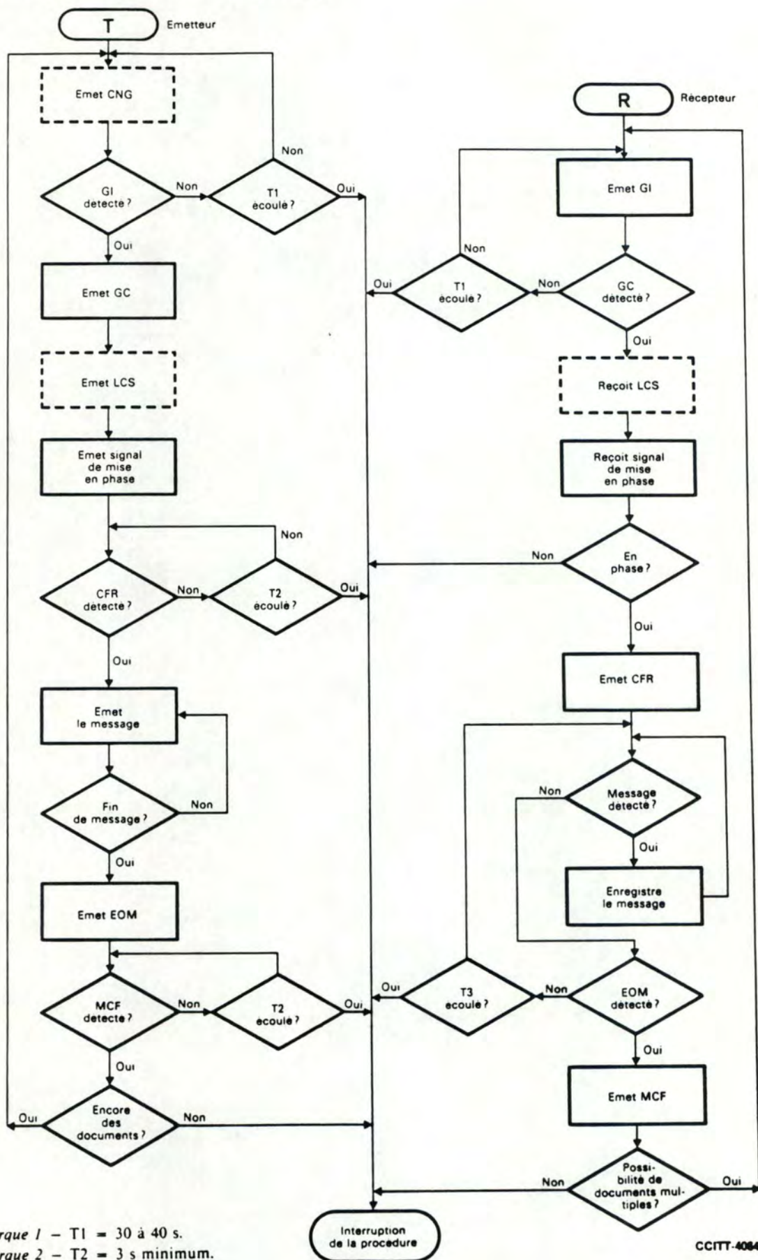
FIGURE 9/T.30
