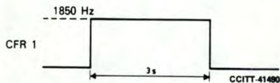
FIGURE 13/T.30
