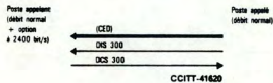
FIGURE V-11/T.30
