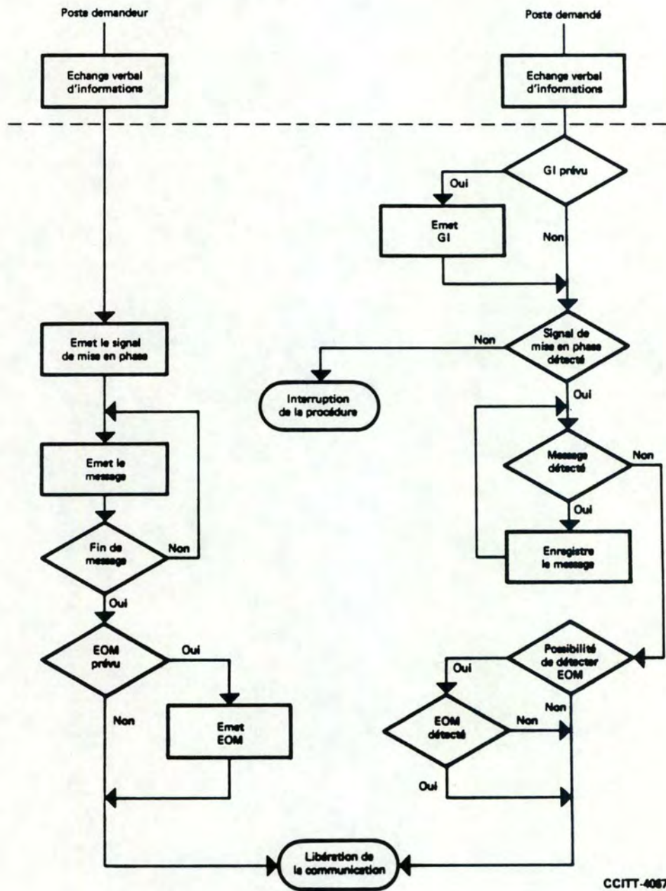
FIGURE I-1/T.30
