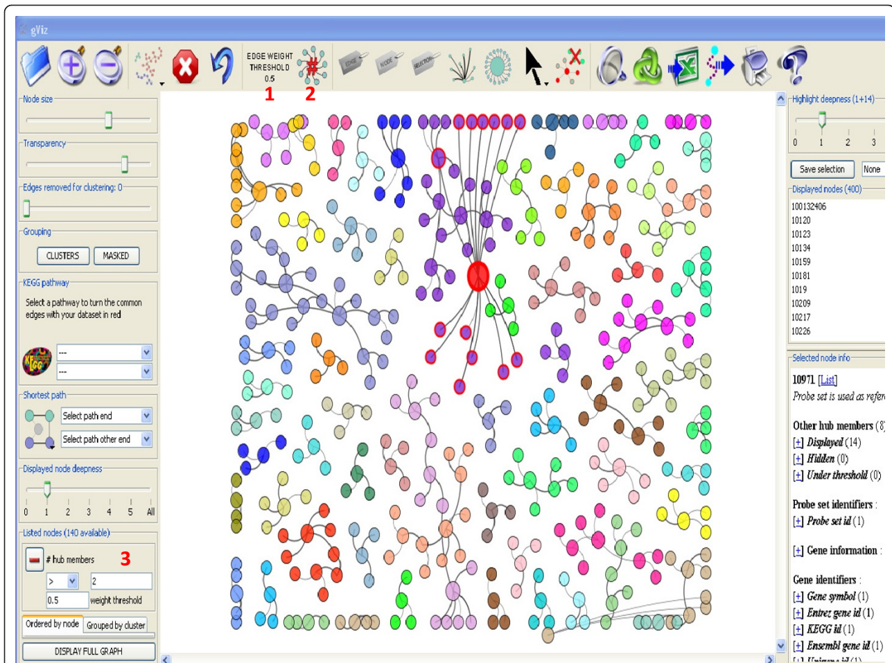
Figure 3 Filters in gViz. This figure displays a network filtered by the number of neighbors ( > 2 ) and the Minet score (score > 0.5 ). The filters are triggered by the buttons in {1} and {2}, and controls for the filters are accessed in the left lower panel {3}.
