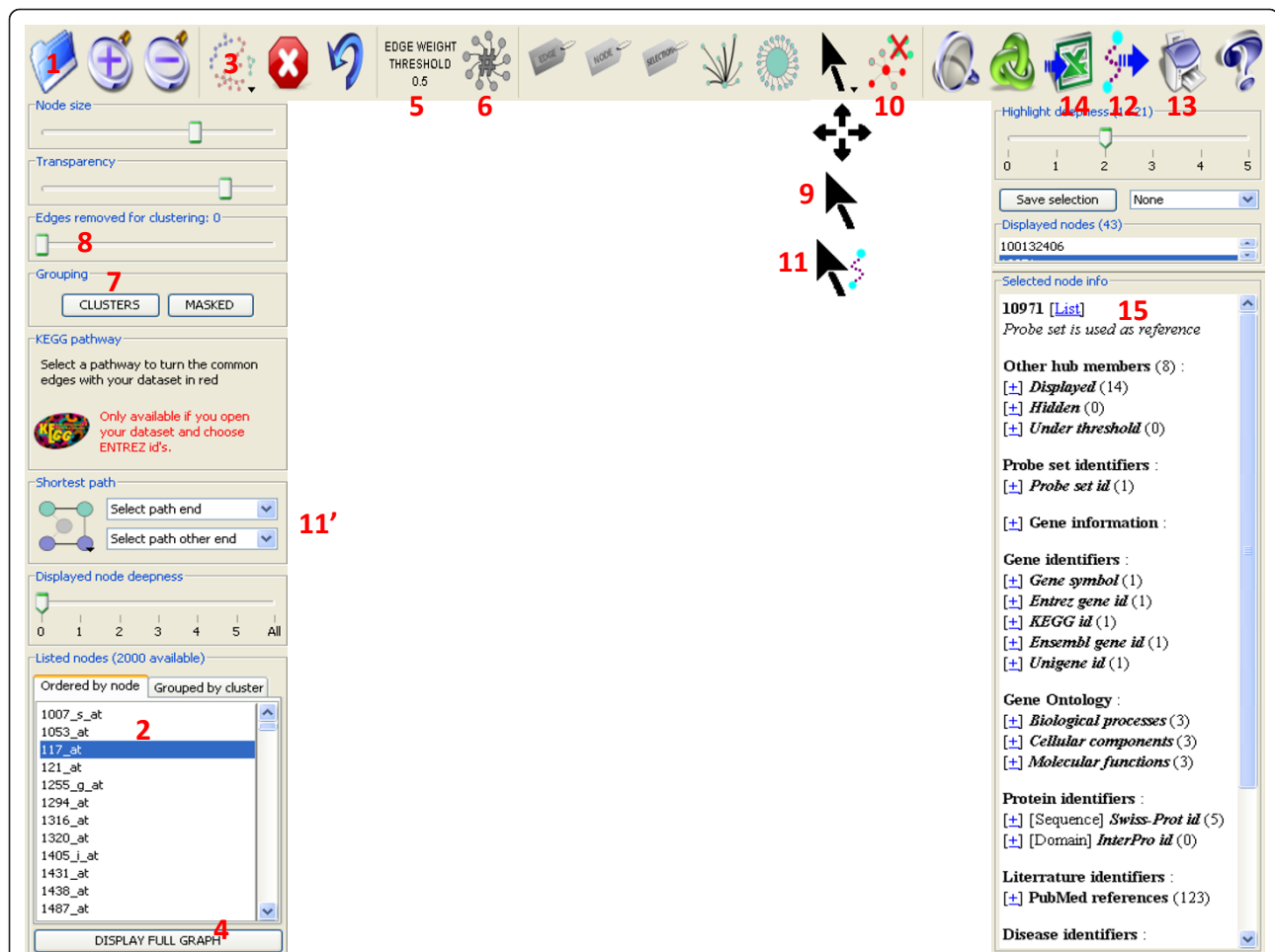
Figure 4 Case study in gViz. Detailed view of the gViz interface and location of the tools mentioned in the 'case study' section. Legend: 1- Open button; 2- Lower left panel, list of nodes available; 3- Layout control button; 4- Display full graph button; 5- Filter on edges scores; 6- Filter on number of neighbors; 7- Clustering button; 8- Edges removed for clustering control slider; 9- Selection tool; 10- Remove non-selected nodes buttons; 11- Shortest path tool; 12- Export shortest path button; 13- Export network (png); 14- Export network (text); 15- Lower right panel, information on selected nodes.
