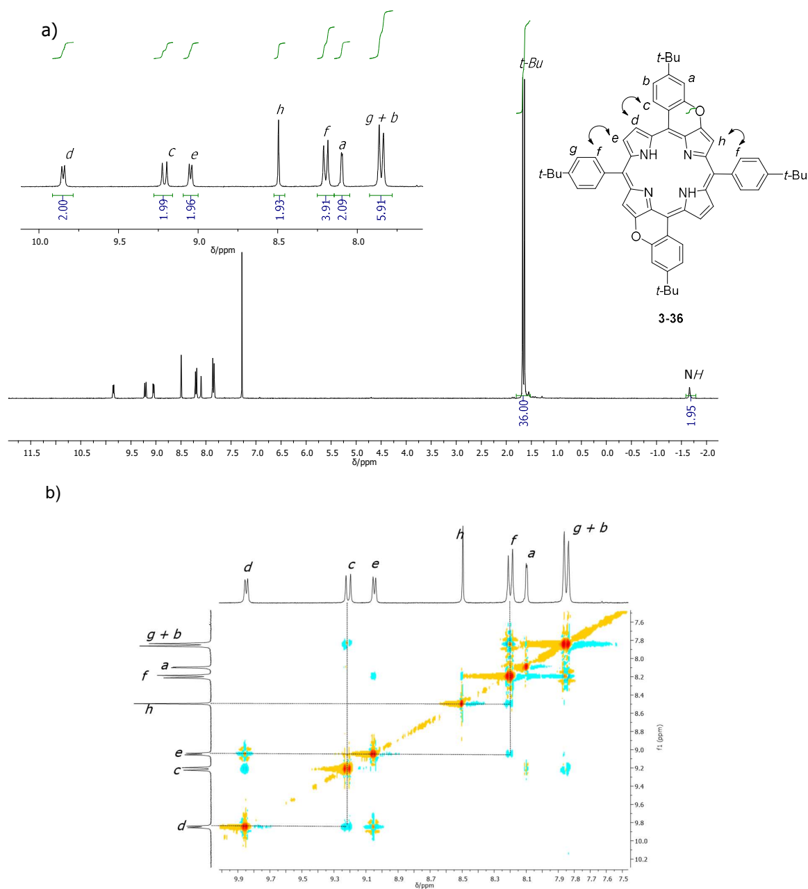
Figure 3.11 NMR analysis of trans -like dipyranoporphyrin 3-36 : a) 1D ^1\text{H} NMR-spectrum (300 MHz, \text{CDCl}_3 ), the inset shows zoom of the 10.00–7.50 ppm area; b) 2D NOESY NMR-spectrum (300 MHz, \text{CDCl}_3 , zoom of the 10.00–7.50 ppm area).
