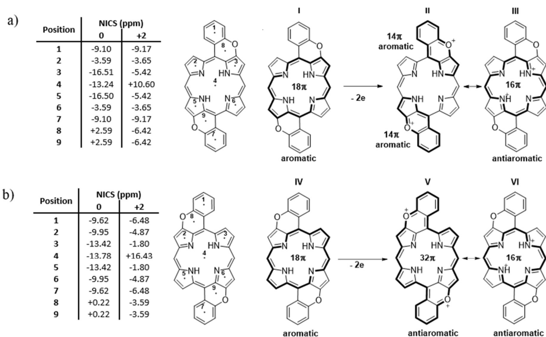
Figure 3.26 Calculated NICS(0) values for the neutral and doubly oxidized trans -like dipyranoporphyryrin tautomers with appropriate aromatic and antiaromatic circuits: a) 3-36a ; b) 3-36b . tert -Butyl groups and meso -(4- tert -butyl)phenyl substituents are omitted.
