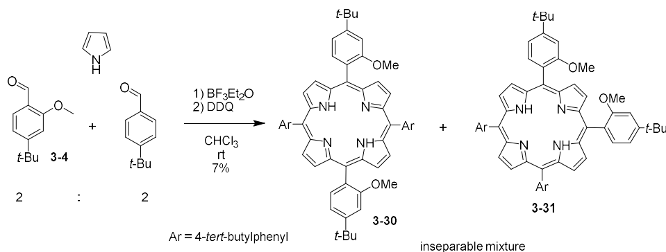
Scheme 3.13 Direct synthesis of dimethoxyporphyrin, resulting in formation of " trans -" and " cis -" isomers 3-30 and 3-31 , respectively.
