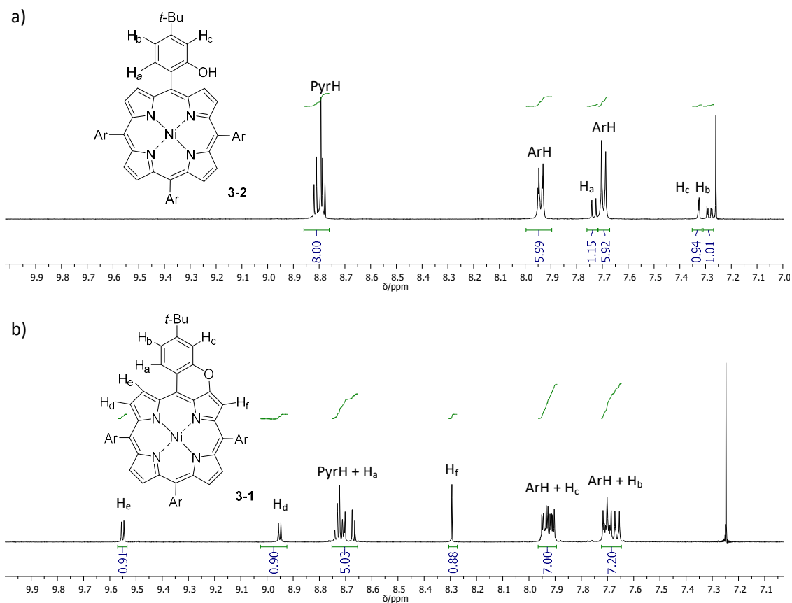
Figure 3.2 ^1\text{H} NMR-spectra of a) monohydroxyporphyrin 3-2 and b) monopyrano-porphyrin 3-1 (400 MHz, \text{CDCl}_3 , zoom of the 10.00-7.00 ppm area), Ar = 4- tert -butylphenyl.
