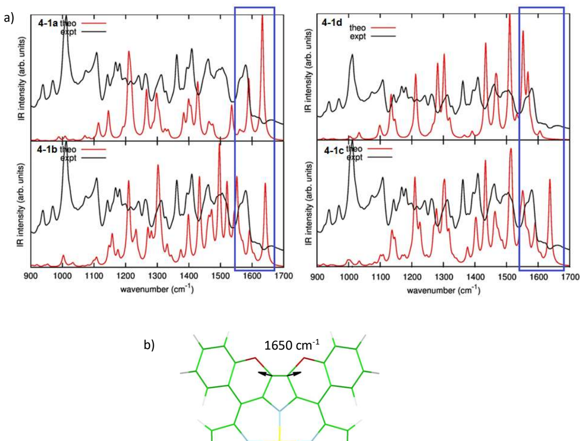
Figure 4.7 a) Comparison of obtained IR spectrum (in black) of 4-1 with calculated IR data (in red) for all possible isomers 4-1a-d ; b) Schematic representation of stretching vibration ( \beta -)C-C( \beta ) bond of a doubly O-fused pyrrole moiety (green C, red O, blue N, yellow Ni).
