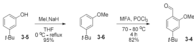
Scheme 3.4 Synthesis of methoxybenzaldehyde 3-4 .
