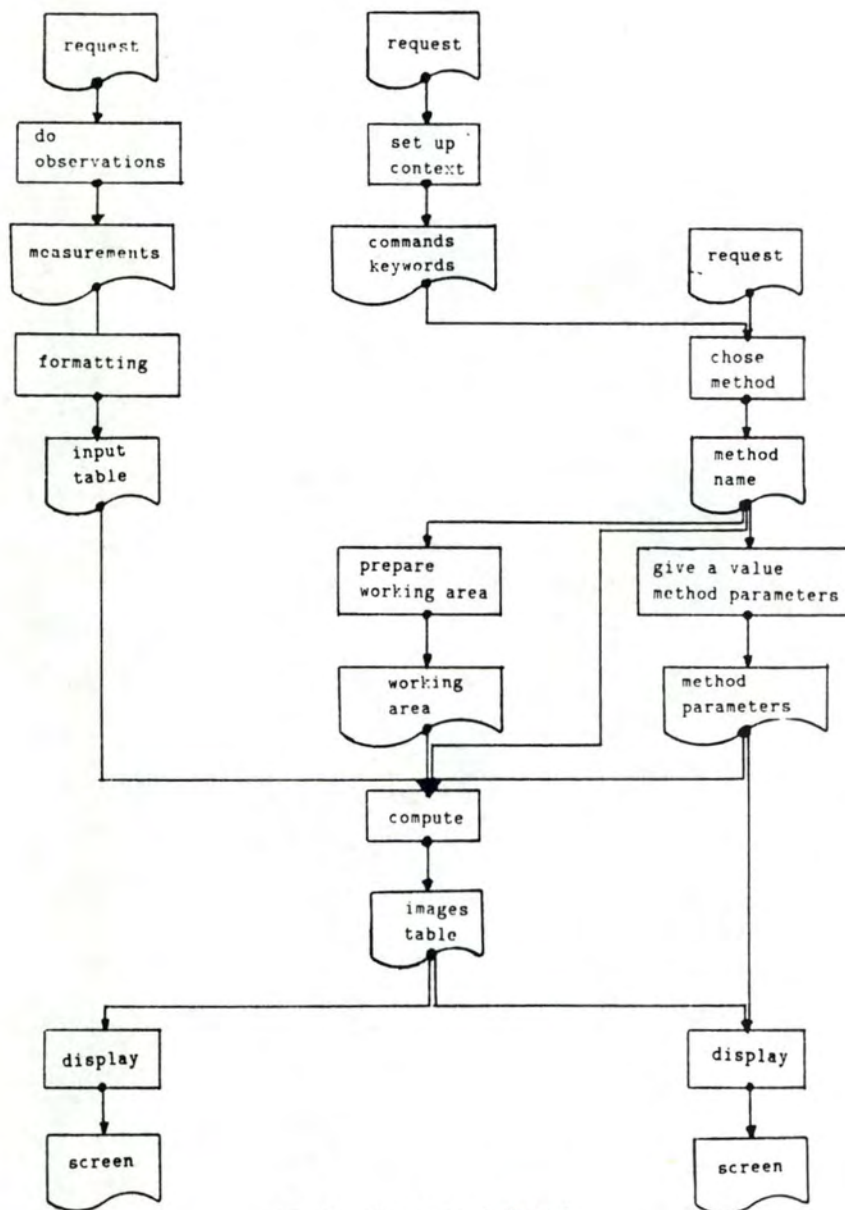
Fig 4.3. The process 's dynamic.
