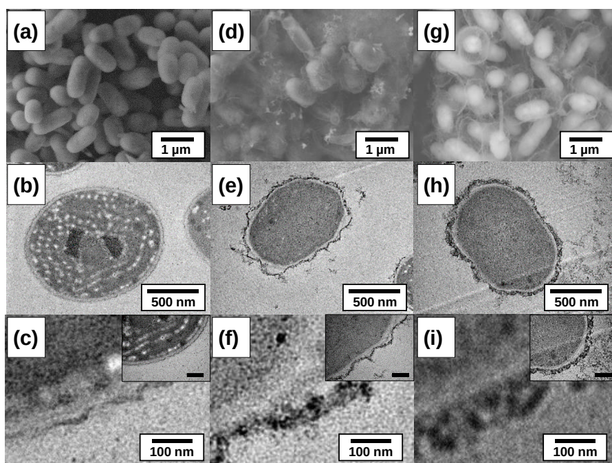
Figure 3: Micrographs of (a), (b) and (c): Free cells; (d), (e), (f) : 2 layers; (g), (h), (i): 4 layers
