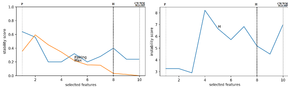
Figure 11.6: Stability graphics obtained with filter method based en cv delta score where selected features is the number of features in the subset.. Graphic on the left is stability score where the higher is the better and the graphic on the right is instability where the lower is ther better. Where Black - is classic wrapper stopping criterion (CW), black – is classic wrapper stopping criterion with margin (WM), black .. is Hoeffding classic (H), grey - is second Hoeffding proposition (H2S), grey – is Hoeffding with permutation (HP) and grey .. is permutation (P)
