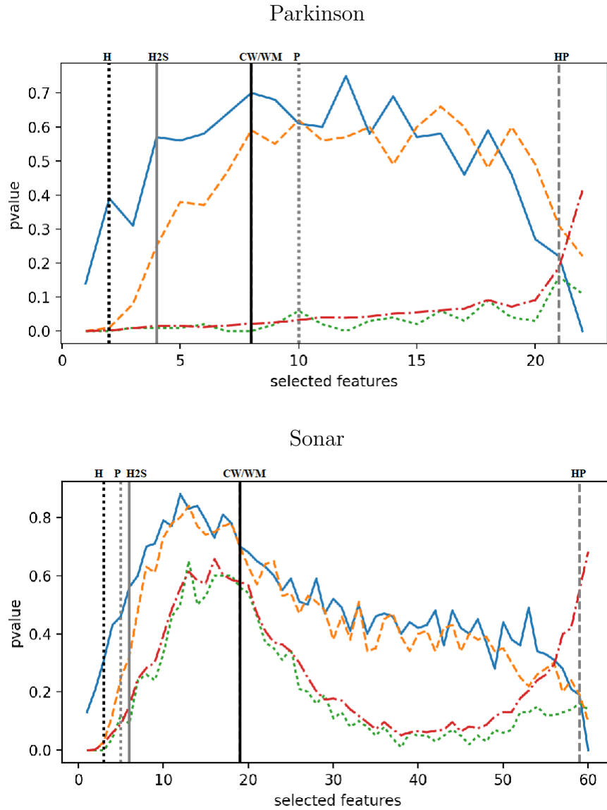
Figure 10.20: p value obtained with forward search base on CV value where selected features is the number of features in the subset. Where - (blue) is the Pvalue of classic hoeffding, - (orange) is the Pvalue of hoeffding S, : (green) is the pvalue of hoeffding P and .- (red) is the value of permutation test
