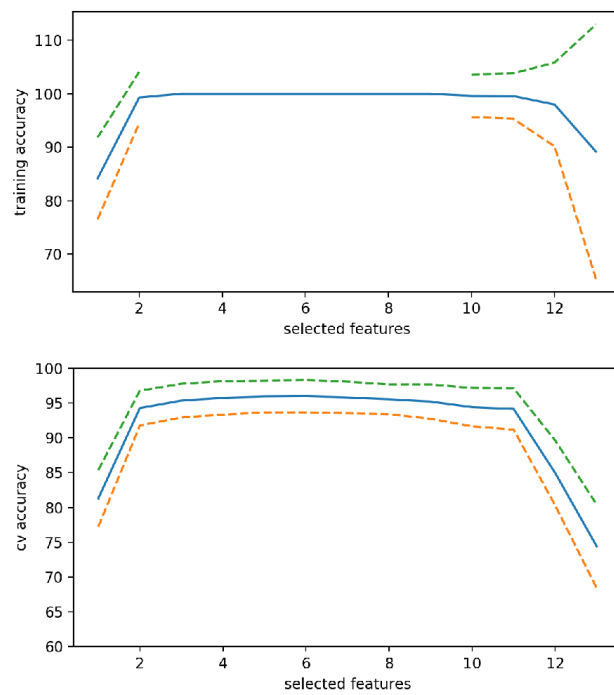
Figure 4.4: Mean of the test Accuracy scores obtained with forward search where selected features is the number of features in the subset. Graphic on the top is training accuracy scores and graphic on the bottom is cv accuracy scores. Dotted line are confidence interval.
