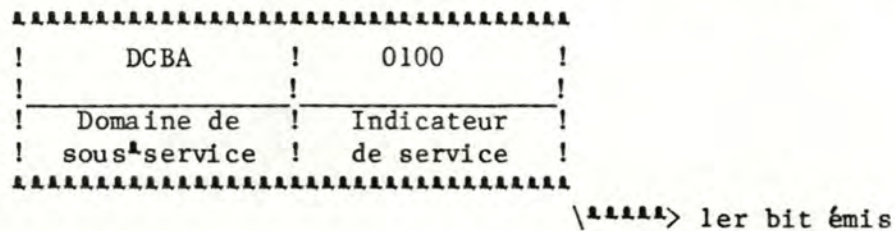
Figure I 1 : Octet de service
