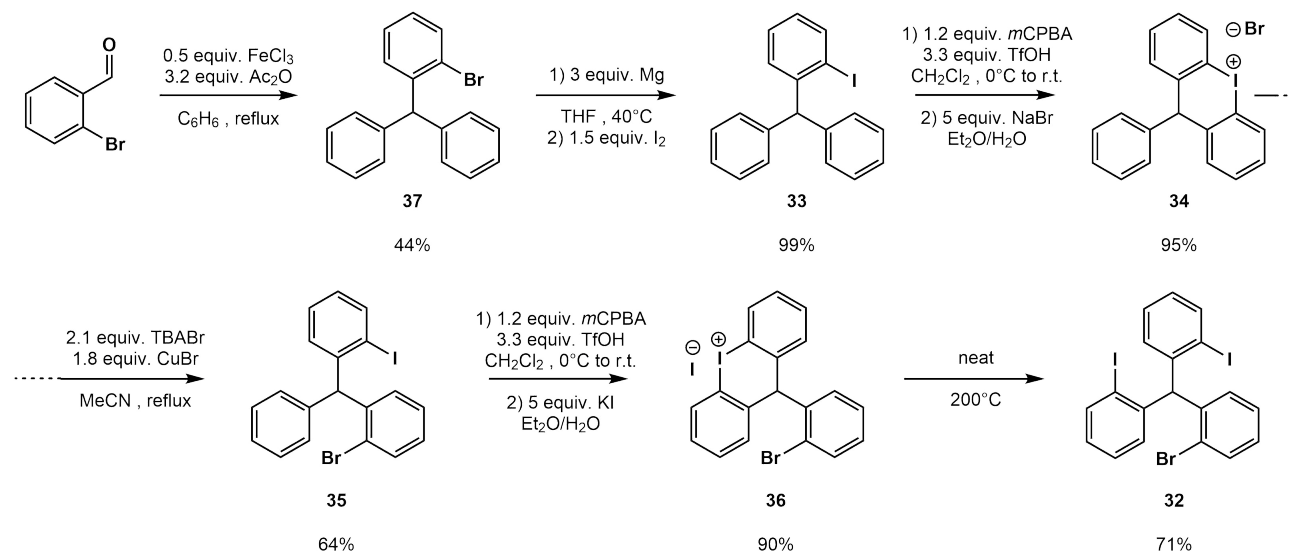
Scheme 3.20: Optimized synthesis of 2,2'-diiodo-2''-bromotriphenylmethane ( 32 )
