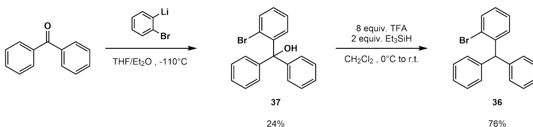
Scheme 3.15: Synthesis of 2-bromotriphenylmethane ( 37 ) using 2-bromophenyl lithium in presence of benzophenone
