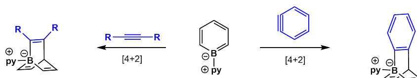
Scheme 3.2: Synthesis of borabarrelene and benzoborabarrelene via Diels-alder addition to borabenzene.
