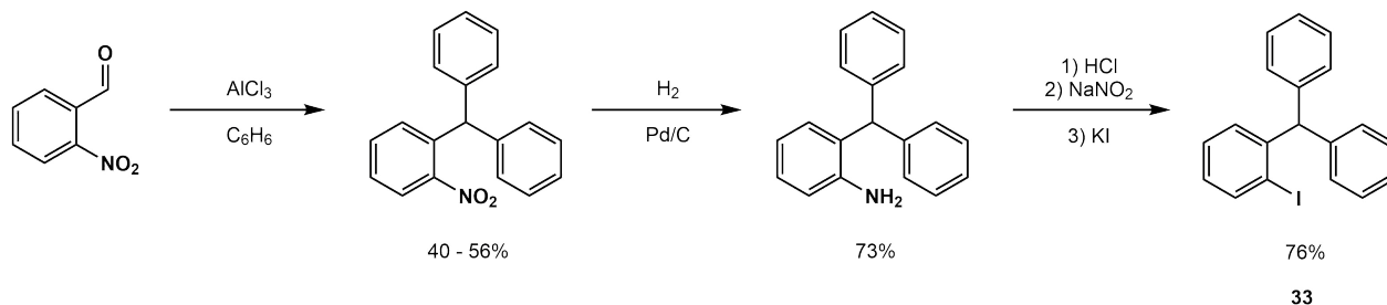
Scheme 3.14: Synthesis of 2-iodotriphenylmethane ( 33 )
