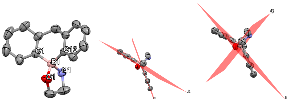
Figure 2.5: X-ray structure of 9-aminoethoxy-9,10-dihydro-9-boraanthracene ( 3 )
