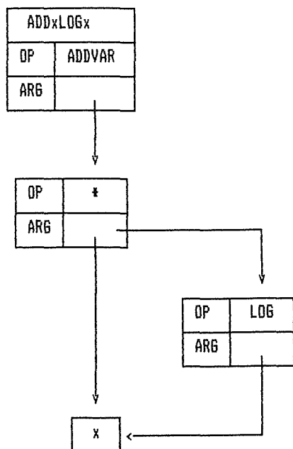
Figure III.1. : Expression \text{ADDxLOGx}
