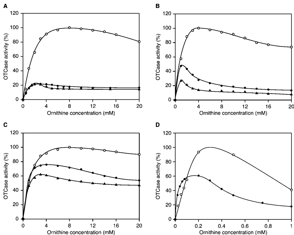
FIG. 5. Inhibition of wild type and mutated OTCases (K260A, K265A, K268A) by wild type arginase as a function of ornithine concentration. The velocity of the reaction catalyzed by wild type and mutated OTCases was measured at 30 °C in 50 mM Tris-HCl buffer, pH 8.0, in the presence of 5 mM CP, 1 mM agmatine, different concentrations of ornithine, and in the presence or absence of wild type arginase. The maximum OTCase activity measured in the absence of arginase was taken as 100%. A , wild type OTCase in the absence of arginase (open circles), in the presence of 200 units of arginase (filled circles), and in the presence of 500 units of arginase (filled triangles). B , OTCase-K260A in the absence of arginase (open circles), in the presence of 200 units of arginase (filled circles), and in the presence of 500 units of arginase (filled triangles). C , OTCase-K265A in the absence of arginase (open circles), in the presence of 200 units of arginase (filled circles), and in the presence of 500 units of arginase (filled triangles). D , OTCase-K268A in the absence of arginase (open circles) and in the presence of 200 units of arginase (filled circles). Note the change of scale in this figure compared with Fig. 5 (A–C).
