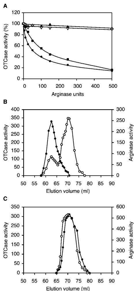
FIG. 7. In vitro inhibition of wild type OTCase by wild type and mutated arginases and elution profiles of a mixture of wild type OTCase and mutated arginases. A, the inhibition test was performed at 30 °C in the presence of 50 mM Tris-HCl, pH 8.0, 15 mM ornithine, and 1 mM agmatine. Wild type arginase (filled circles), arginase-H309K, H312E (filled squares), arginase-C321R, C326T (filled triangles), and arginase-H309K, H312E, C321R, C326T (open triangles). B, elution profile of a mixture of 3200 units of wild type OTCase (open circles) with 900 units of mutated arginase-H309K, H312E (filled circles) in the presence of 15 mM ornithine and 1 mM agmatine. C, elution profile of a mixture of 3200 units of WT OTCase (open circles) and 2500 units of mutated arginase-C321R, C326T (filled circles), in the presence of 15 mM ornithine and 1 mM agmatine.
