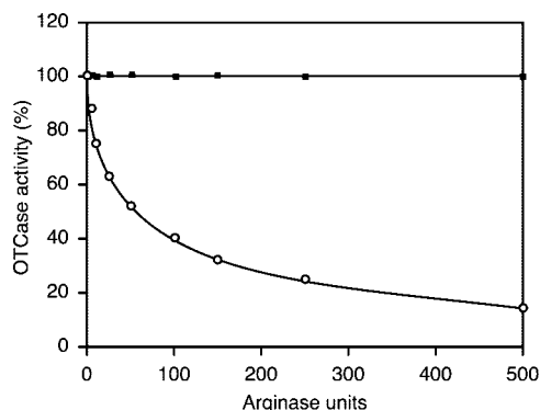
FIG. 2. In vitro inhibition of wild type OTCase and mutated OTCase-D182N by wild type arginase. The inhibition test was performed at 30 °C in the presence of 50 mM Tris-HCl, pH 8.0, 15 mM ornithine for the wild type OTCase and 200 mM for the D182N variant, 1 mM agmatine, and increasing amounts of arginase (4). Maximum OTCase activity measured in the absence of arginase was taken as 100%. Open circles, WT OTCase; filled squares, OTCase-D182N.
