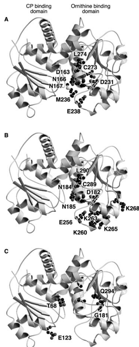
FIG. 4. View of the \alpha -carbon chain of the predicted structure of the OTCase monomer from S. cerevisiae using the structure of the E. coli OTCase as template. A, E. coli OTCase monomer taken from the crystal structure reported by Ha et al. (34). Residues interacting with ornithine are indicated. Secondary structure elements: \alpha helices are represented by cylinders, and \beta strands are represented by arrows. B, S. cerevisiae OTCase monomer modeled on the basis of the structure of E. coli OTCase. Residues required for regulation by arginase are indicated. C, S. cerevisiae OTCase monomer. Residues whose changes did not affect the OTCase-arginase interaction are indicated.
