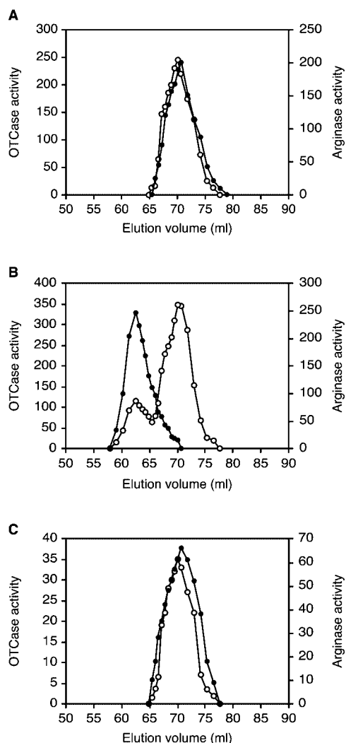
FIG. 3. Elution profile of a mixture of arginase and OTCase extracted from wild type and mutant strains. The molecular mass of arginase is about 114 kDa and that of OTCase is about 120 kDa (A). When the two enzymes are associated as in B, the molecular mass of the associated peak is about 200 kDa. Arginase and OTCase from wild type and mutant strains were eluted on Superdex 200 column with Tris-HCl 50 mM, pH 8.0. A, elution profile of 2400 units of WT OTCase (open circles) and 1000 units of WT arginase (filled circles), in the absence of ornithine and agmatine. B, elution profile of a mixture of 3400 units of WT OTCase (open circles) and 900 units of WT arginase (filled circles), in the presence of 15 mM ornithine and 1 mM agmatine. C, elution profile of a mixture of 400 units of mutant OTCase D182N (open circles) and 500 units of WT arginase (filled circles), in the presence of 200 mM ornithine and 1 mM agmatine.
