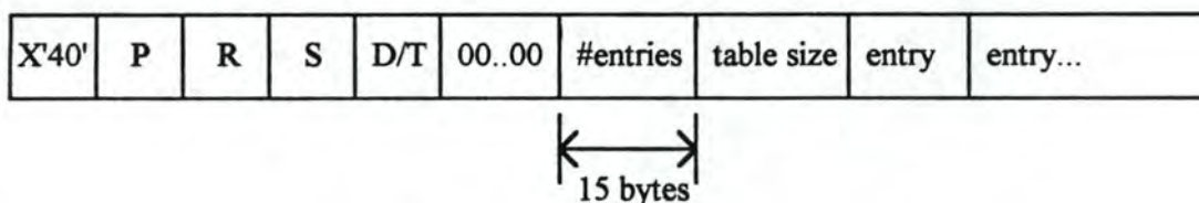
Figure 3.2 - Structure of record in RSO parameters file
