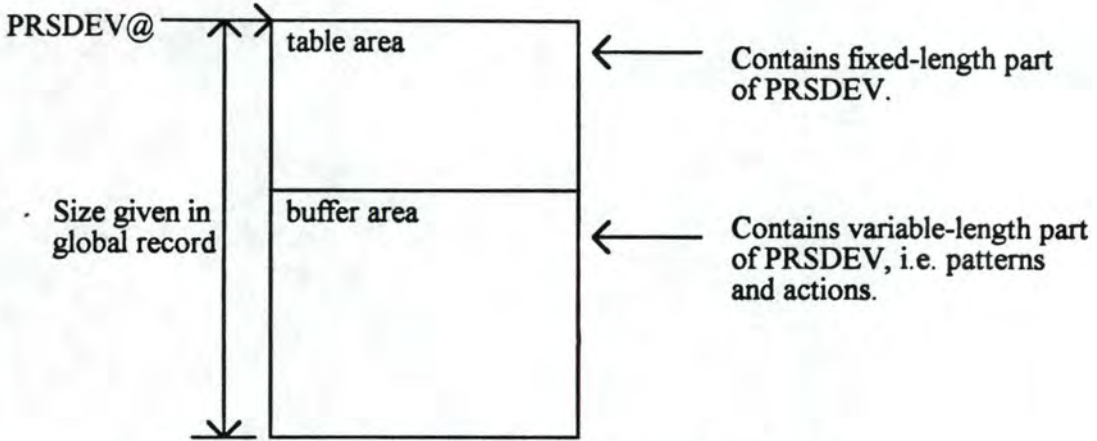
Figure 3.5 - Split structure of PRSDEV table
