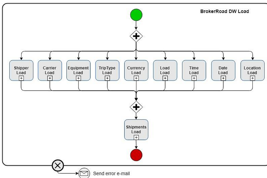
Figure 4.1 : orchestration du processus ETL
