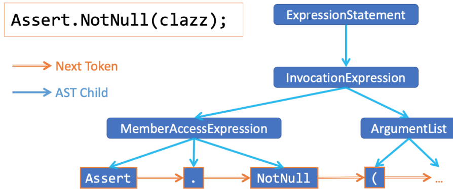
Figure 8.5: AST comes with blue arrows and adding the orange arrows makes it graph, reproduced from https://miltos.allamanis.com/files/slides/2019fosdem.pdf
