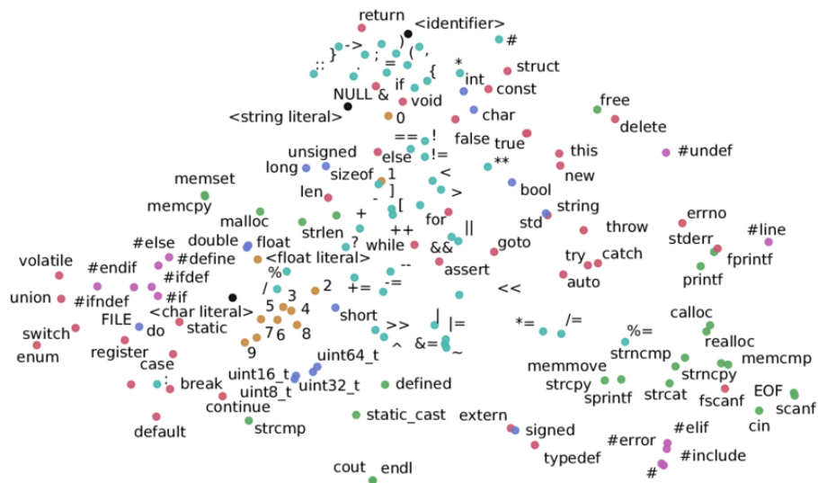
Figure 6.4: Embedding of C# tokens, reproduced from [A. Harer et al., 2018]
