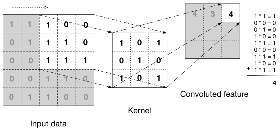
Figure 5.3: The kernel sliding over the top-right part of the image, adapted from "Deep Learning" by Adam Gibson, Josh Patterson
