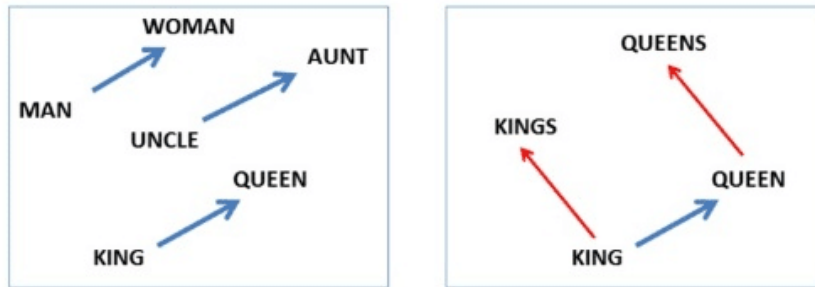
Figure 6.3: Property of word2vec, from [Mikolov et al., 2013]
