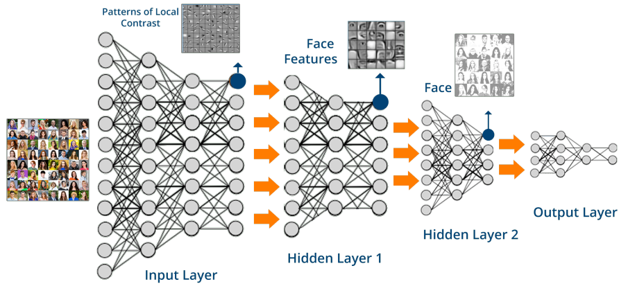
Figure 5.2: The features more and more identifiable being extracted by the network.
