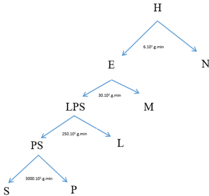
Figure 33: Simplified scheme of the subcellular fractionation protocol. The first centrifugation of the homogenate at 6.10^3 \text{ g.min} will give the nuclear fraction (N) and the supernatant is the cytoplasmic extract (E). This one undergoes a series of centrifugation at higher and higher speed giving the heavy mitochondrial fraction (M) at 30.10^3 \text{ g.min} the light mitochondrial fraction (L) at 250.10^3 \text{ g.min} , and the microsomal fraction at 3000.10^3 \text{ g.min} . The soluble fraction (S) contains all cell component non-sedimentable at the speed of 3000.10^3 \text{ g.min} . LPS and PS are supernatants containing the corresponding fractions.
