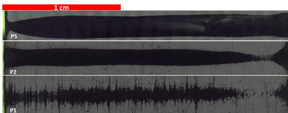
Figure 6. Stitched microscopic images of PA joint area after failure (dark areas), illustrating effect of laser-ablation parameters on joint quality.
