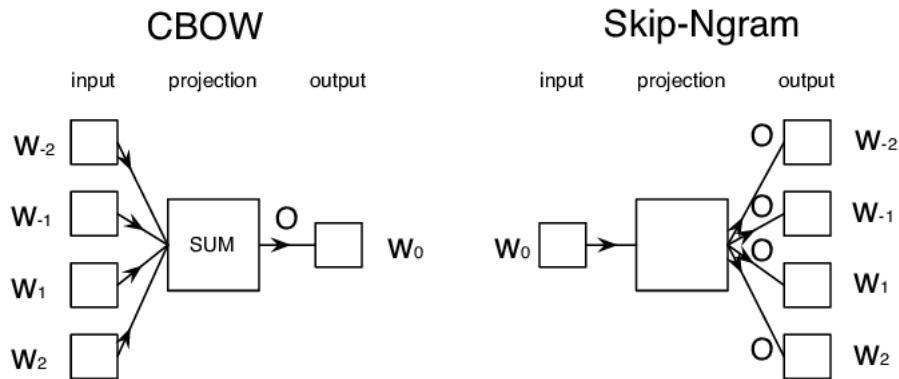
Figure 1.8: Architecture CBOW et Skip-Gram [Bornstein, 2018]
