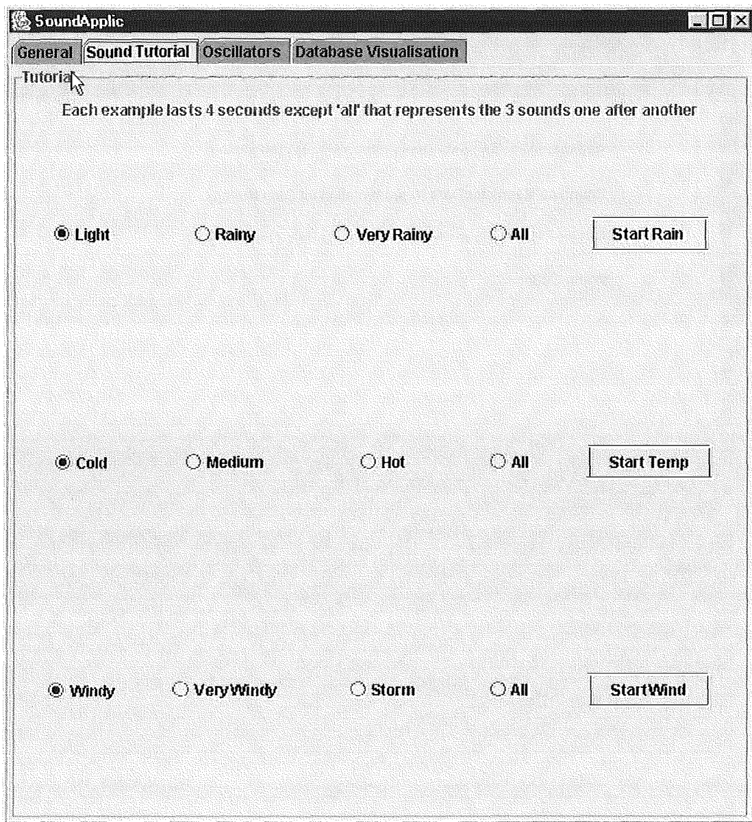
Figure 8.3: SoundApplic, Sound Tutorial
