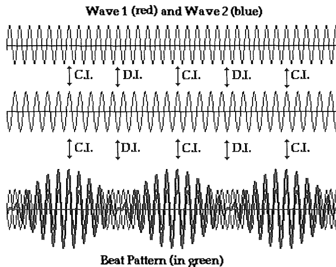
Figure A.4: Beat pattern
