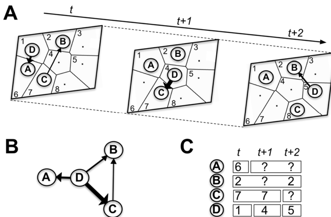
Figure 2. Schematic representations of Call Detail Records (CDRs) data. Letters (A–D) represent SIM cards (~individuals), numbers (1–8) represent antenna coverage approximated by a Voronoï tessellation, and arrows represent call direction (head) and duration (width). (A) geo-spatial, dynamic, directed weighted network (here weights are call duration), (B) static, directed weighted network (over t to t + 2 period), and (C) dynamic trajectories of SIM cards.
