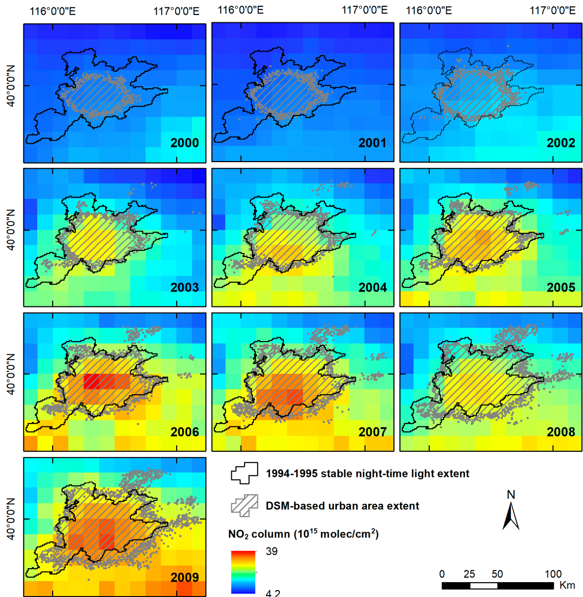
Figure 16. Yearly tropospheric NO 2 columns, with a posting of 7.5 arc minutes (GCS WGS 1984), overlapped by the corresponding Beijing DSM-based urban area (dashed gray areas) for each year in the 2000s. The “filtered” Beijing 1994–1995 stable night light extent [20] (black contour) is overlaid on all datasets as a common and consistent spatial reference area.
