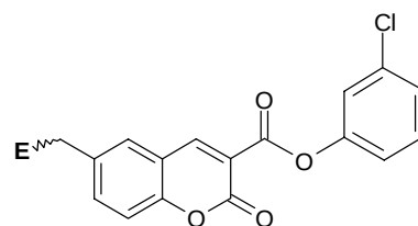
alkyle-enzyme
