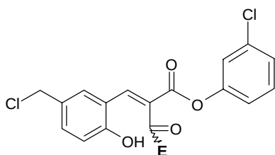
acyle-enzyme
