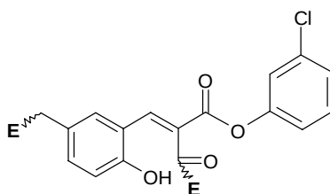
alkyle-enzyme biponté
