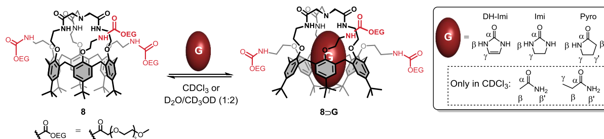
Scheme 2. Host-guest properties of calix[6]cryptamide 8 towards polar neutral guests.
