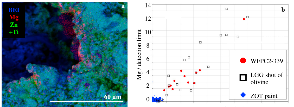
Fig. 4. Small impact WFPC2-339: a) BEI and SEM-EDX maps show Mg-rich residue concentrated in thin frozen frothy paint melt, lining the impact pit ; b) plot shows higher Mg and Fe levels in spectra of impact melt (red circles) than in clean ZOT paint (blue diamonds); and similar to residue from LGG of olivine grains (open black squares).
