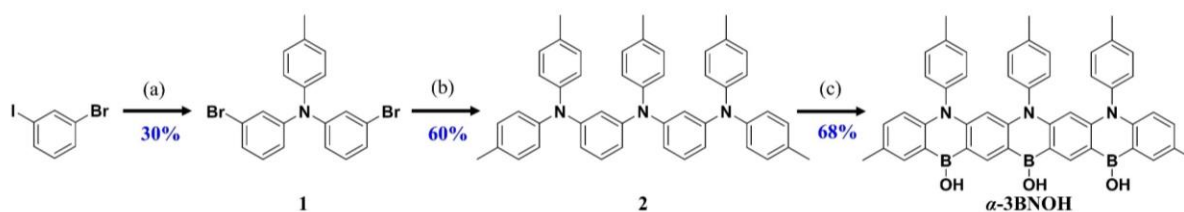
Scheme 1. Synthesis of \alpha -3BNOH. a) p -toluidine, Cu, CuI, K 2 CO 3 , reflux 5 days b) di- p -tolylamine, Pd(OAc) 2 , [( t -Bu) 3 PH]BF 4 , NaOt-Bu, toluene, 110 °C, 24 h c) BBr 3 , 1,2-4-trichlorobenzene, 200 °C, 12 h.
