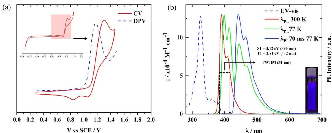
Figure 4. Solution-state optoelectronic measurements of \alpha -3BNOH. a) Cyclic and differential pulse voltammograms measured in degassed THF with 0.1 M [n\text{Bu}_4\text{N}]\text{PF}_6 as the supporting electrolyte and \text{Fc}/\text{Fc}^+ as the internal reference (0.28 V vs. SCE). 56 Scan rate = 100 \text{ mV s}^{-1} b) Absorption, steady-state at 300 K and emission at 77 K (steady-state and with 70 ms delay) measured in THF and steady-state emission at 300 K measured in PMMA (1 wt% emitter) spin cast film. \lambda_{\text{exc}} = 325 \text{ nm} . Inset figure shows PL of \alpha -3BNOH in THF at 300 K.
