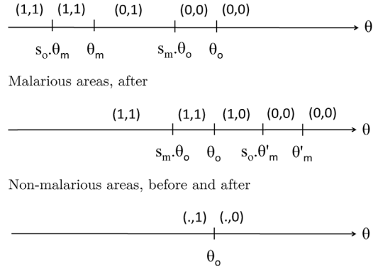
Fig. A.3. Health investments ( x_m^* , x_0^* ) before and after subsidizing anti-malaria products.
