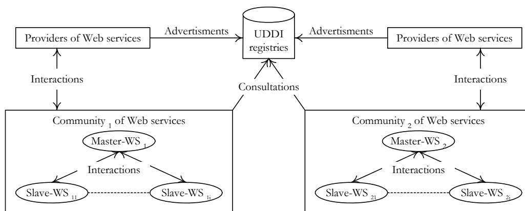
Figure 1 Architecture of single Web services communities per functionality
