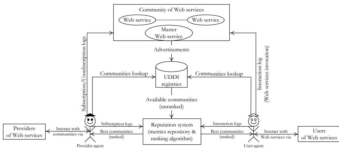
Figure 2 Architecture of multiple Web services communities per functionality
