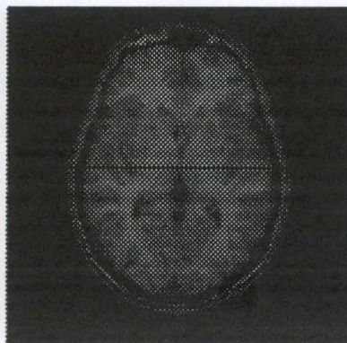
Figure 2: MR image
