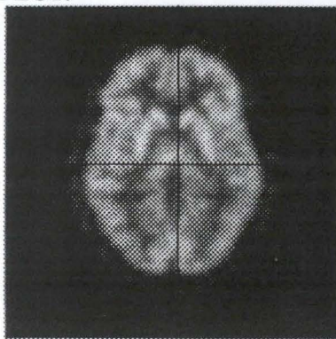
Figure 1: PET image
