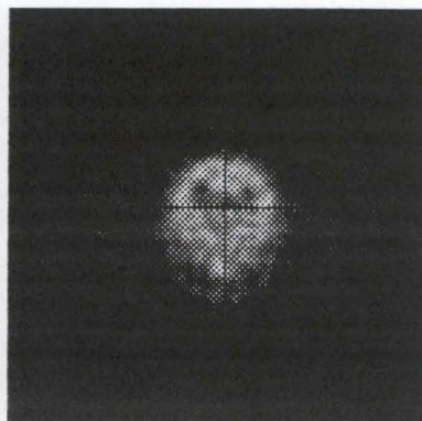
Figure 3: SPECT image
