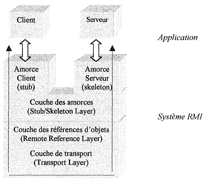
Figure 5.1. Architecture de RMI
