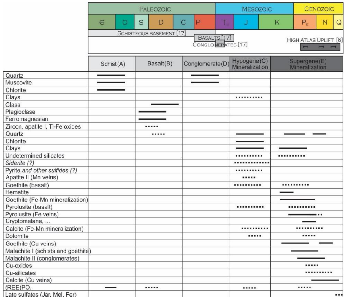
Figure 5.2.8. Paragenese of Jbel Rhals rocks and mineralization, in relation to the evolution of the geological/geodynamical context: (A) formation of the Paleozoic schisteous basement; (B) Permo-Triassic basalts flow; (C) alteration of the host rocks, basalts, and formation of a hydrothermal ore; (D) Triassic conglomerates; (E) weathering probably related to the High Atlas Uplift. Relative ages of the formations are from Chefchaoui et al. (1963), and of the High Atlas uplift from Leprêtre et al. (2015).
