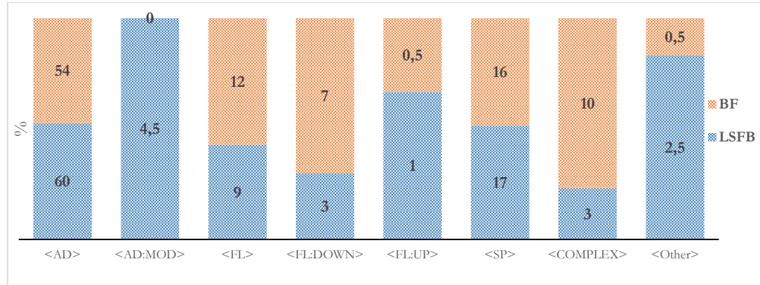
Fig. 44: Distribution in percent of gaze direction types by language.
