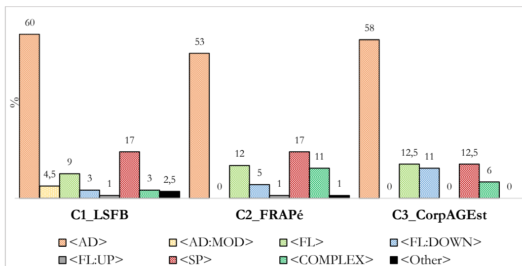
Fig. 45: Distribution in percent of gaze direction types by corpus.
