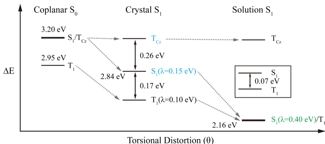
Figure 5. Summary of CMA1 phase-dependent photophysics. At the coplanar S 0 geometry (identical for solution and solid phases), S 1 and T Cz are quasidegenerate, while at the solution S 1 geometry (featuring complete torsional distortion), S 1 and T 1 are quasidegenerate. While the 0.4-eV reorganisation energy of S 1 in solution leads to a large energy gap with respect to the negligibly changed (< 0.1 eV) T Cz state, the smaller 0.15-eV reorganisation energy of the partially rotated S 1 in the crystal leads to a 0.26-eV energy gap with respect to T Cz that is comparable to the T 1 -S 1 energy gap of 0.17 eV at this geometry. The state labels have been coloured to reflect the emission energy ranges from these states, where observed experimentally. The inset details the results from multireference orbital optimisation for the non-solid-phase (solution) T 1 geometry of CMA1 in isolation.
