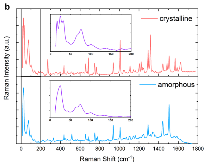
Figure 1: a X-ray diffraction of crystalline and amorphous CMA1. Three distinct peaks appear at 8.2, 8.7 and 10.3 degrees. The inset shows weak crystallisation of annealed PEO (100,000) with two peaks at 19.2 and 23.4 degrees. b Raman spectra of crystalline and amorphous CMA1. Raman shift below 200\text{ cm}^{-1} is magnified. Films were drop cast from CMA1 chlorobenzene solution (20 mg/ml) mixing with 20 wt.% PEO (Mw 100,000 Da) in a nitrogen glovebox, followed by annealing at 120\text{ }^{\circ}\text{C} for 1 min to crystallise.
